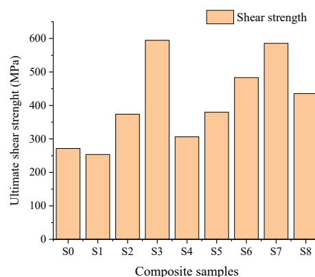
Fig 1. Ultimate Shear Strength of Composite Sample
